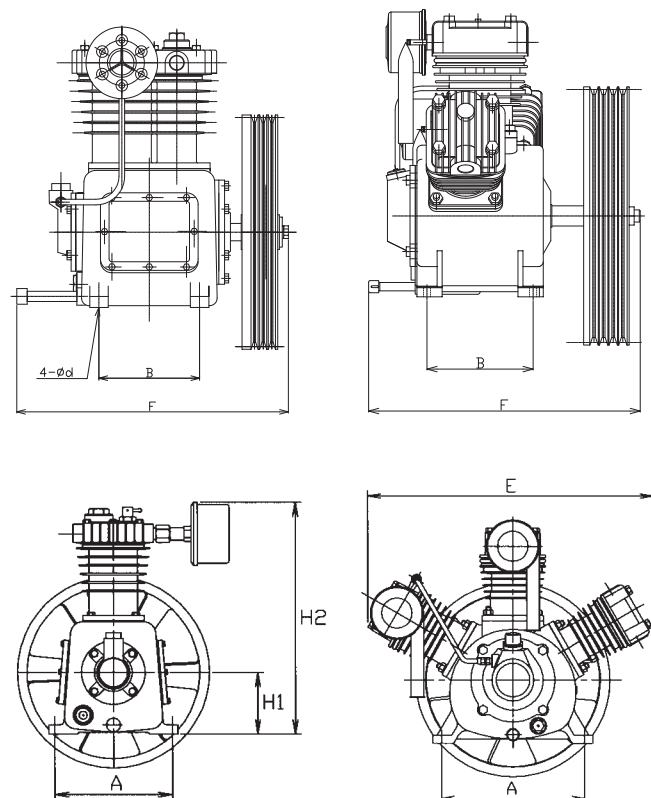
寸法図 OW-33D・OW-35D～OW-110H
